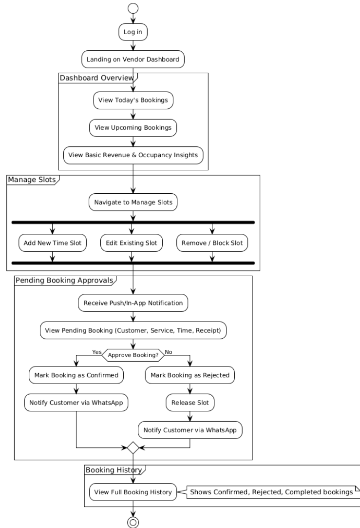
Figure 4.6: Activity Diagram: Vendor Dashboard & Approvals
