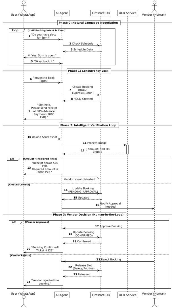
Figure 4.3: AI Booking & Payment Pipeline
