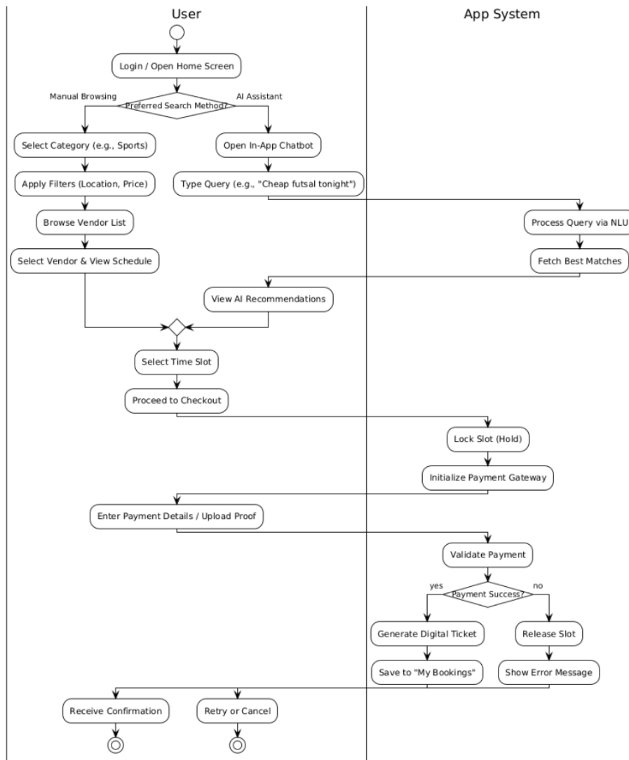
Figure 4.5: Activity Diagram: Mobile App Search & Book
